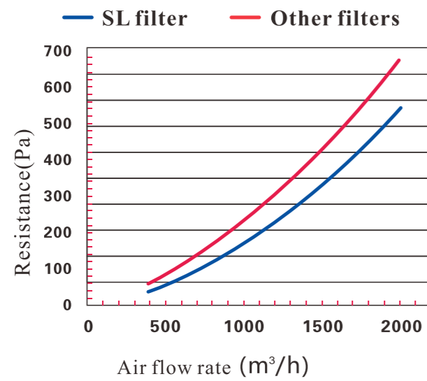
The plot of flow rate against the resistance
